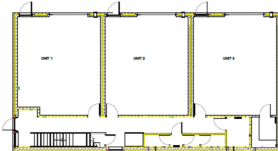
GROUND FLOOR LAYOUT 1:50
